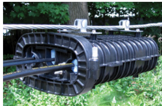
Low Clearance Strand Mounting Bracket
